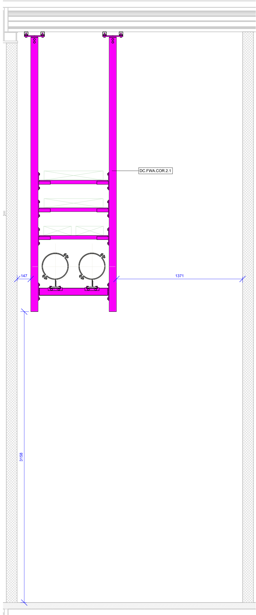
2 | Building 1 - Supports - First Floor - East Corridor 2 - Section 2
