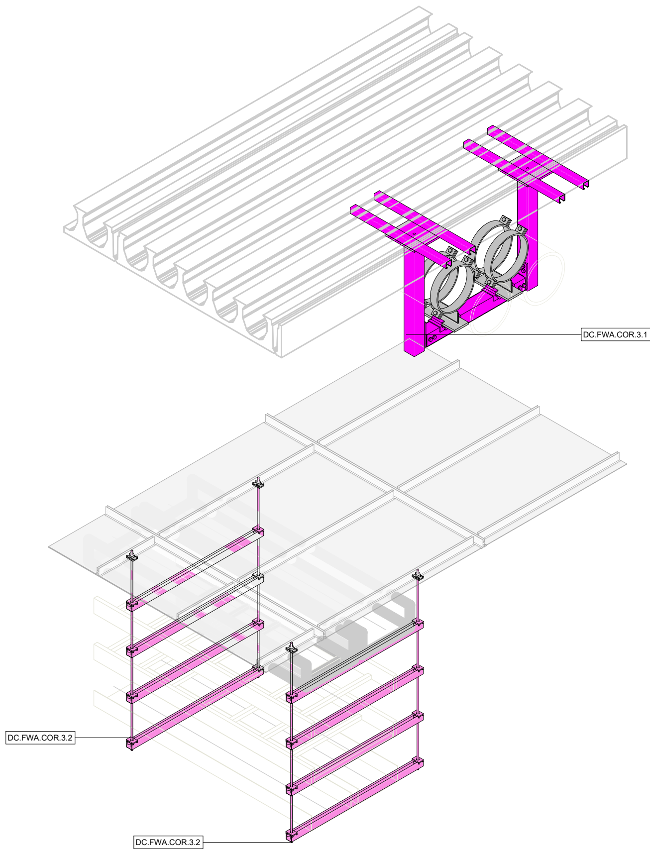
3D1 | Building 1 - Supports - First Floor - West Corridor 3 - 3D ISO
