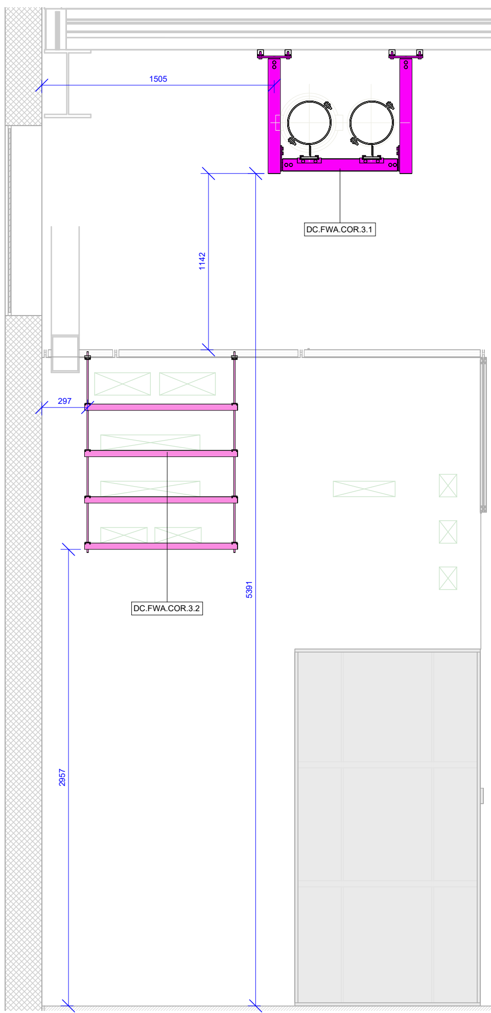
3 | Building 1 - Supports - First Floor - West Corridor 3 - Section 3
