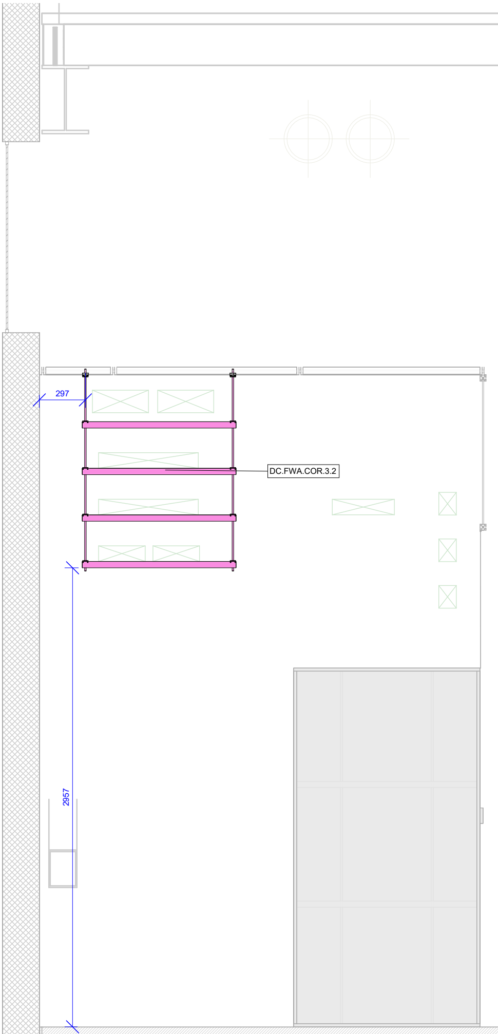
2 | Building 1 - Supports - First Floor - West Corridor 3 - Section 2
