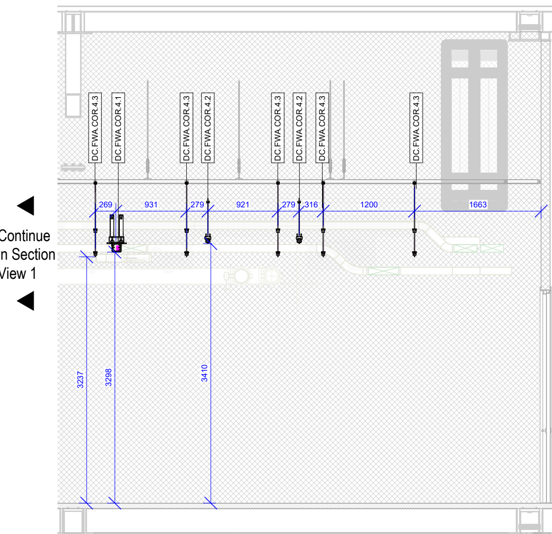
2 | Building 1 - Supports - First Floor - North Corridor 4 - Section 2
