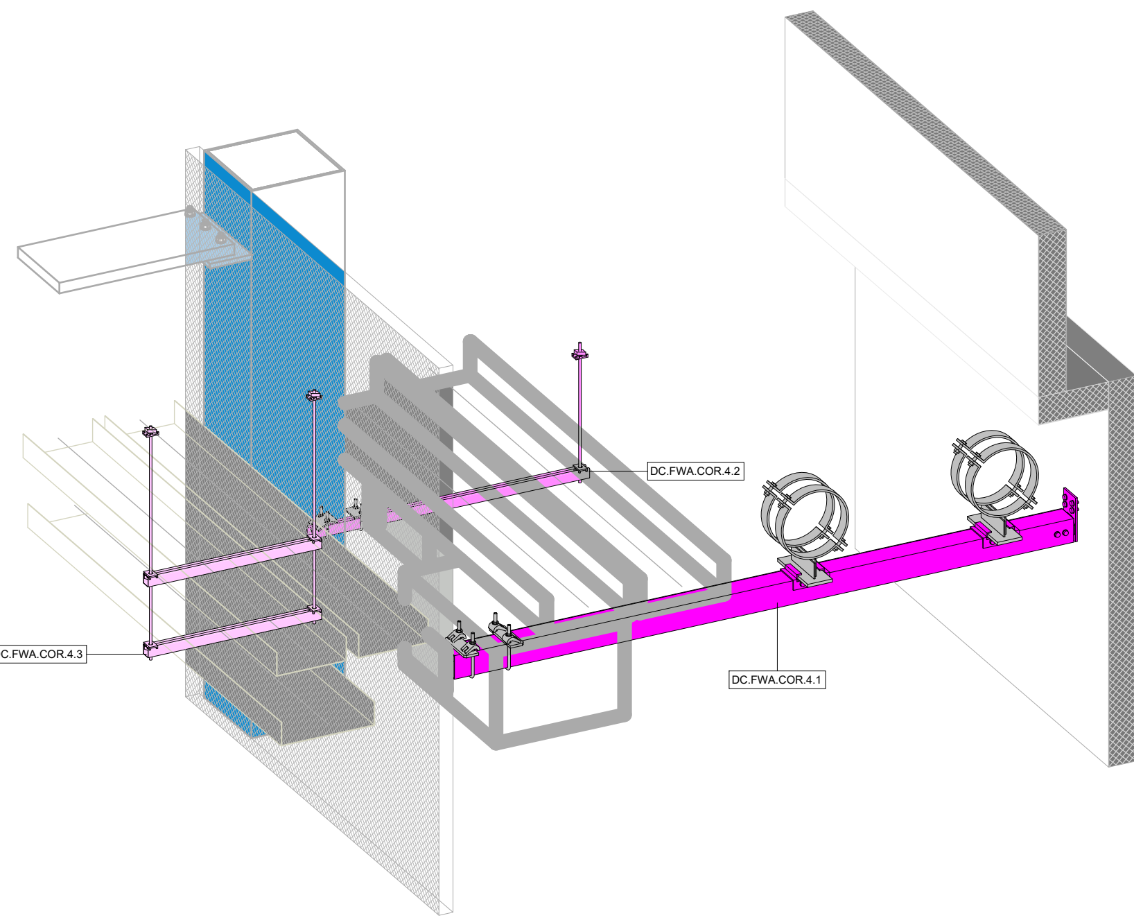
6 | Building 1 - Supports - First Floor - North Corridor 4 - 3D ISO
