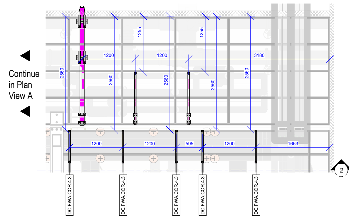
B | Building 1 - Supports - First Floor - North Corridor 4 - Plan View B
