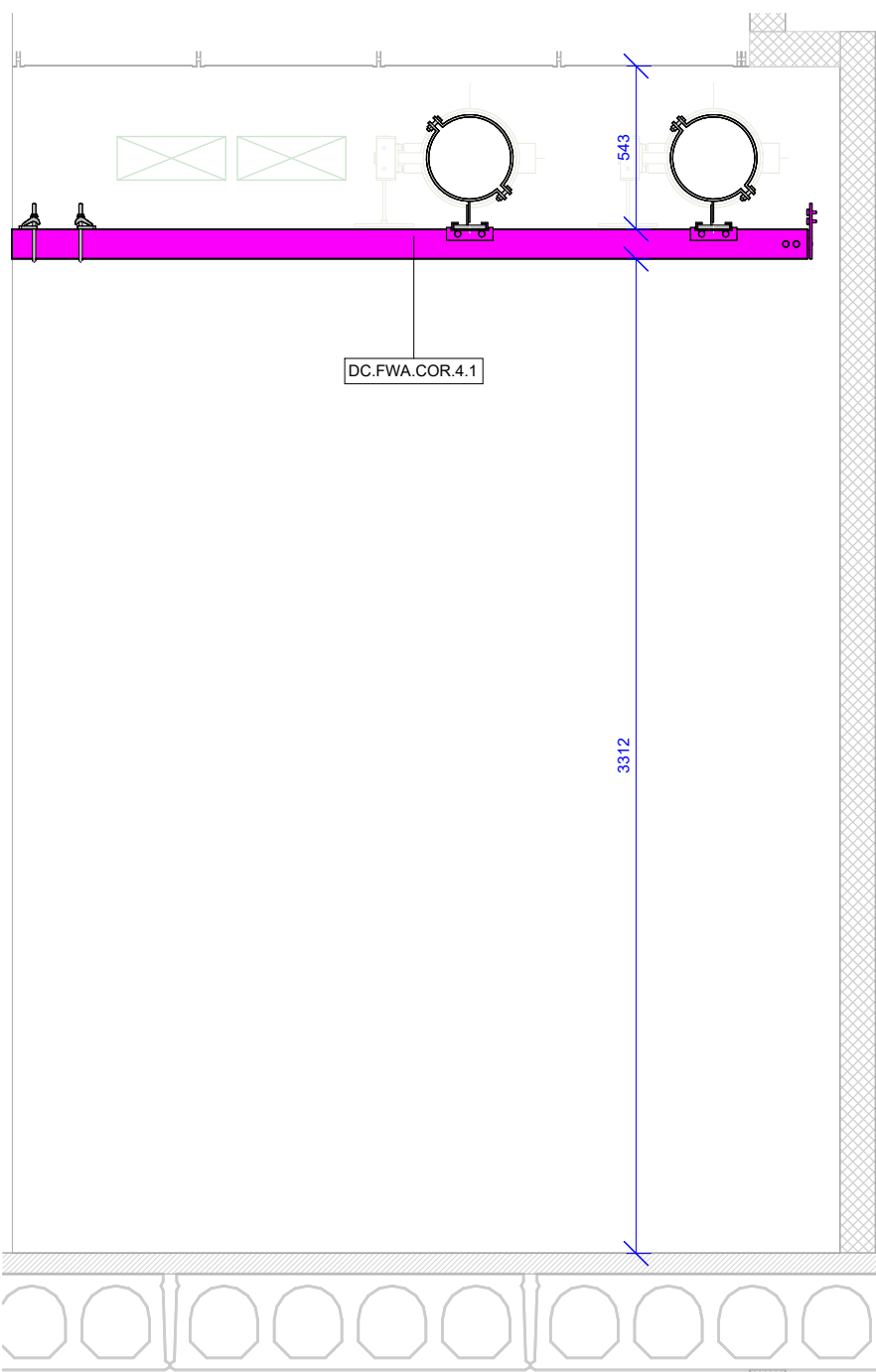
3 | Building 1 - Supports - First Floor - North Corridor 4 - Section 3
