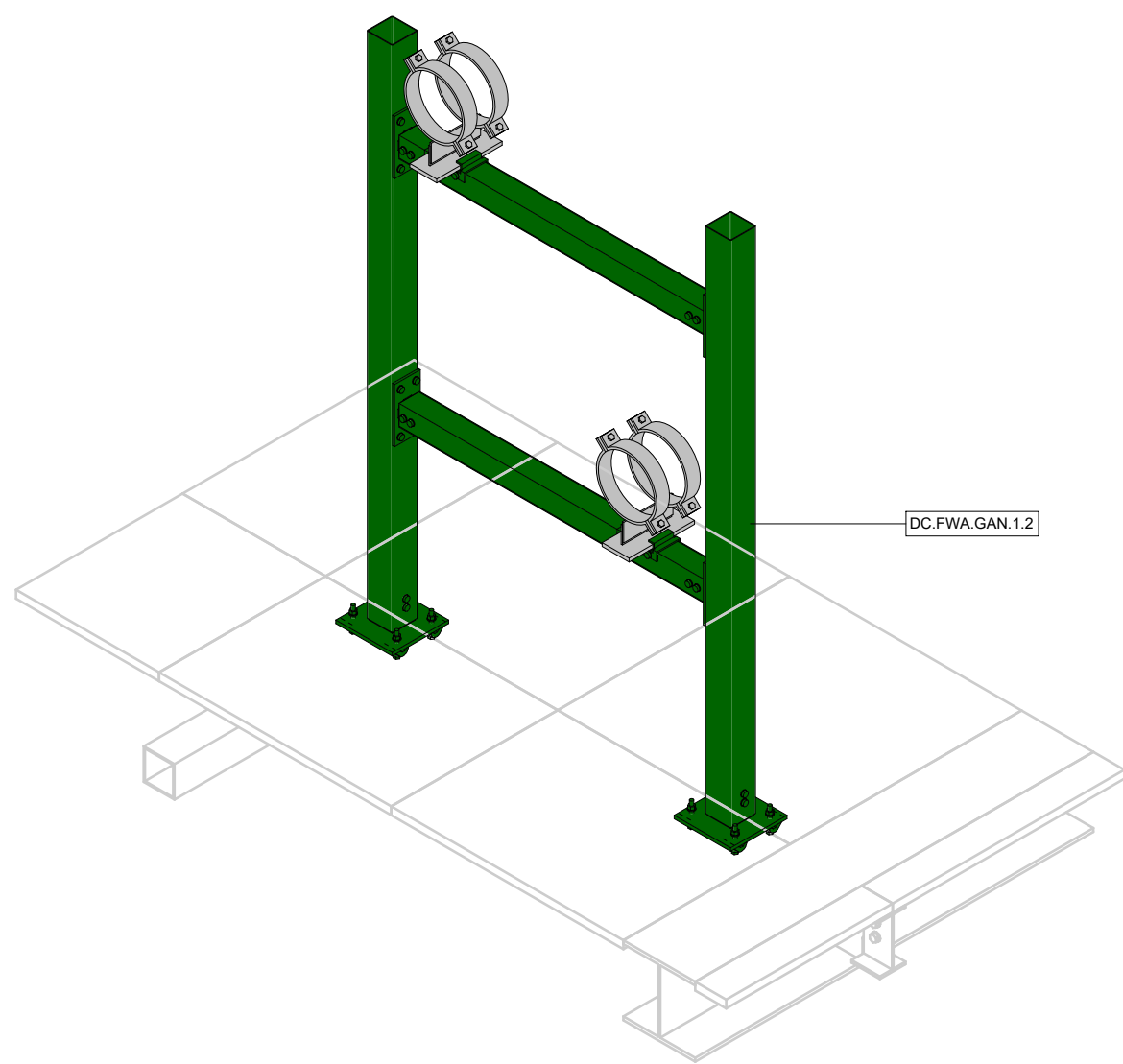
3D2 | Building 1 - Supports - North Gantry - Zone 01 - 3D ISO 02
