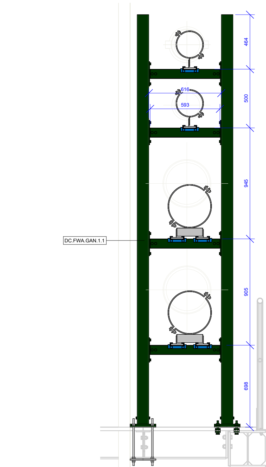
3 | Building 1 - Supports - North Gantry - Zone 01 - Section 3
