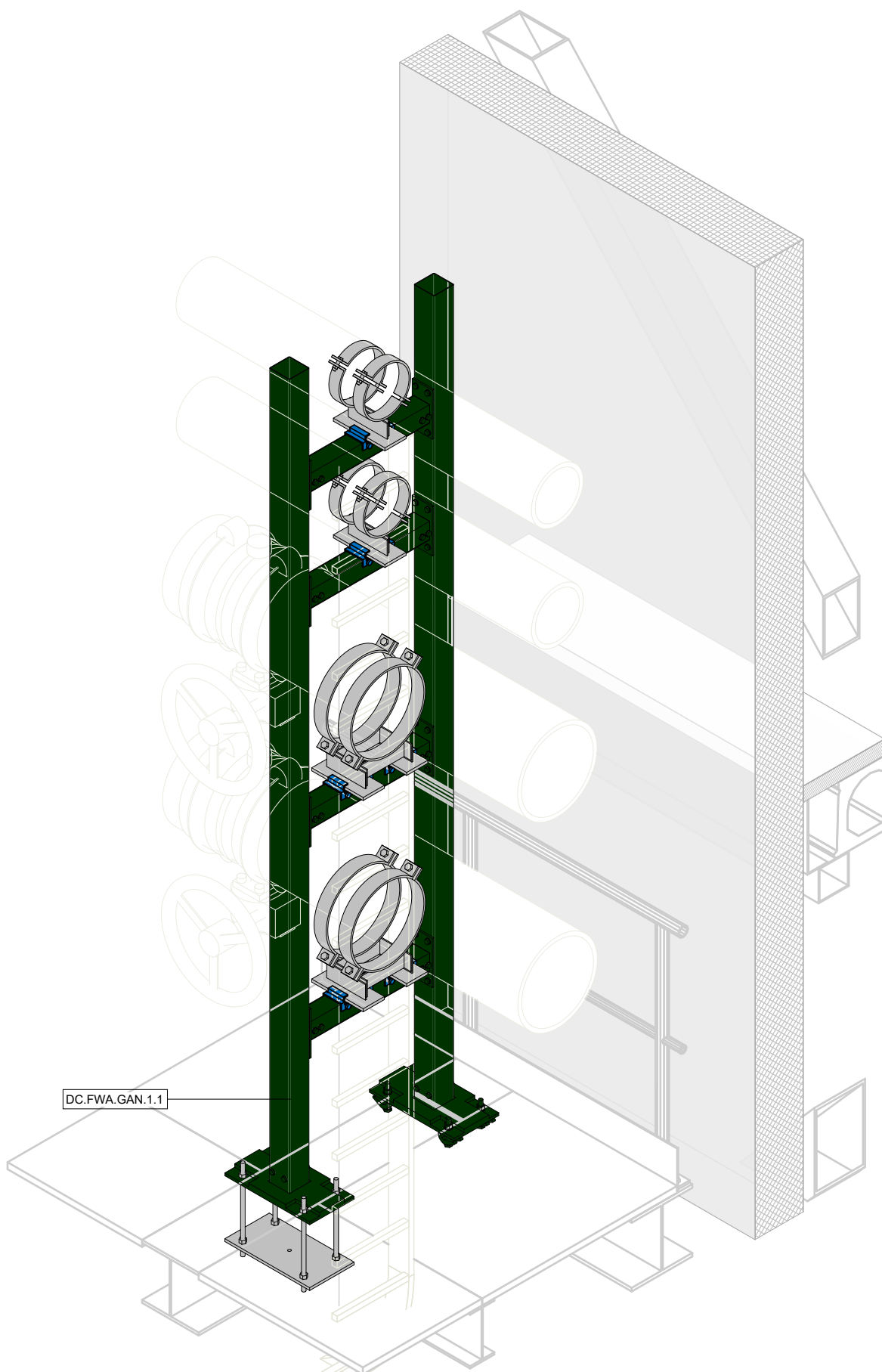
3D1 | Building 1 - Supports - North Gantry - Zone 01 - 3D ISO 01
